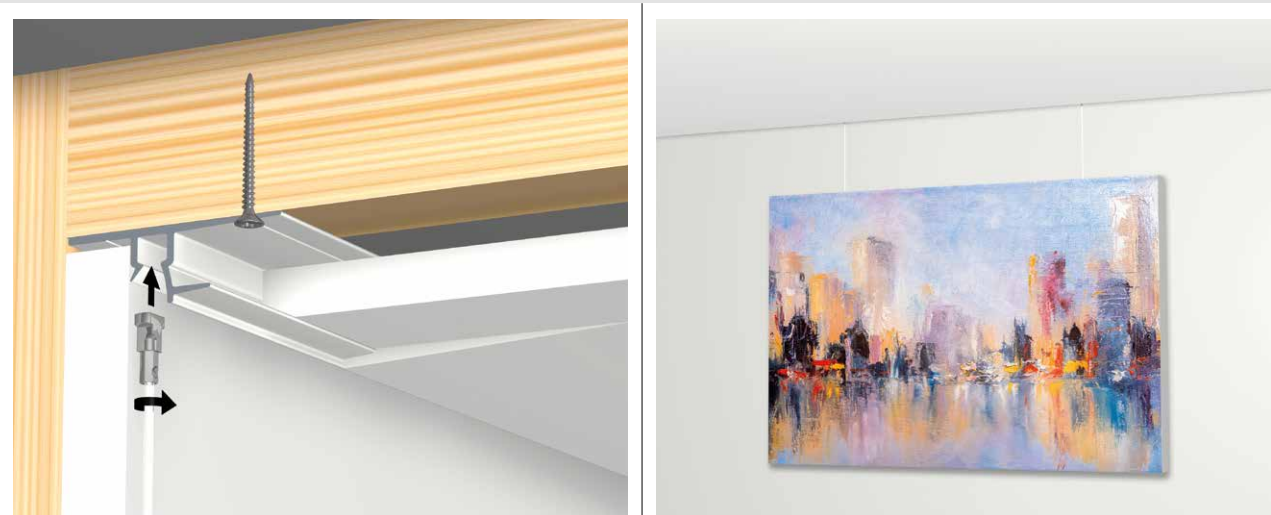
SHADOWLINE DRYWALL (IN COMBINATION WITH DRYWALL)
